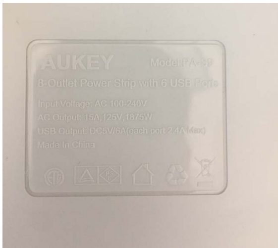
Product Nameplate
